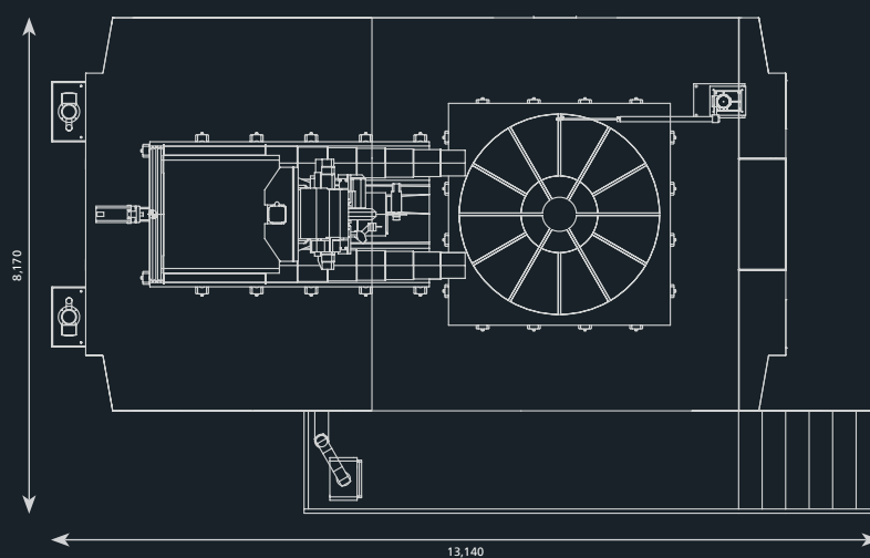
RAPID 6000: Top View
