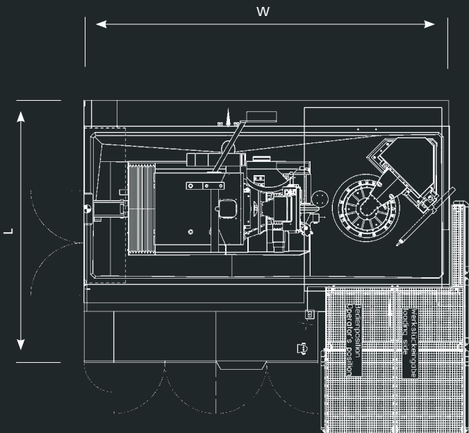
RAPID 650–800 (L/XL): Top View
