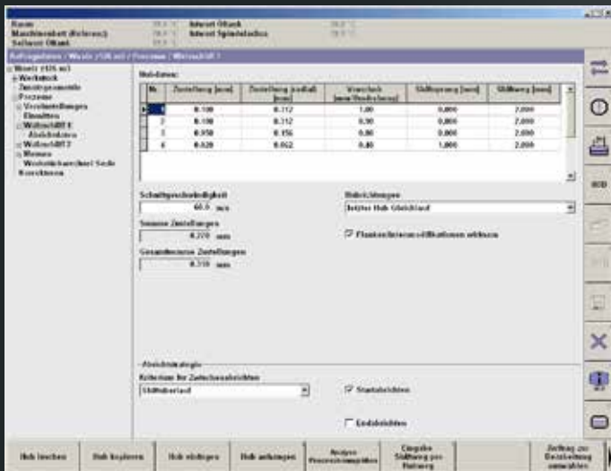
Input of process data for generating grinding
