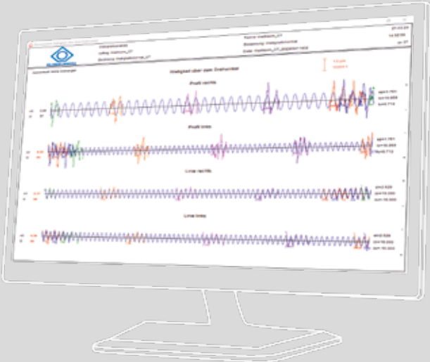
Evaluation of profile, flank and pitch using the extended standard measurement (4+4)
