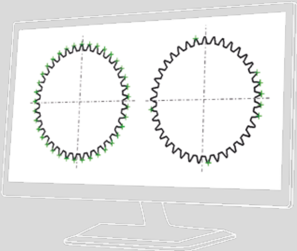
Schematic view of the all-tooth measurement (left) and the extended standard measurement 4+4 (right)
