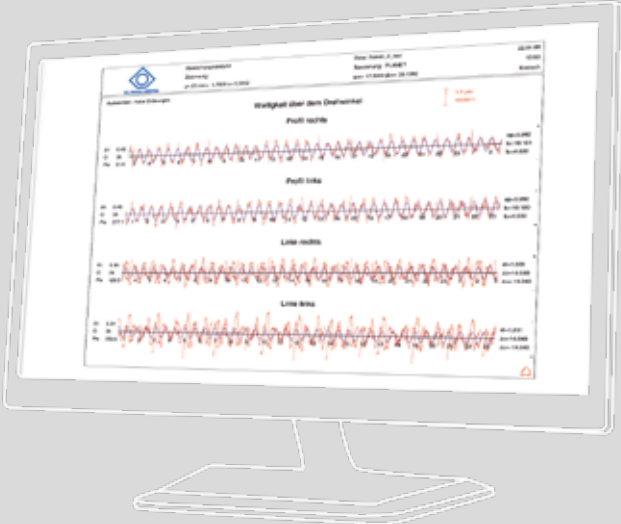
The combined display of deviation curves for a loud gear teeth.
