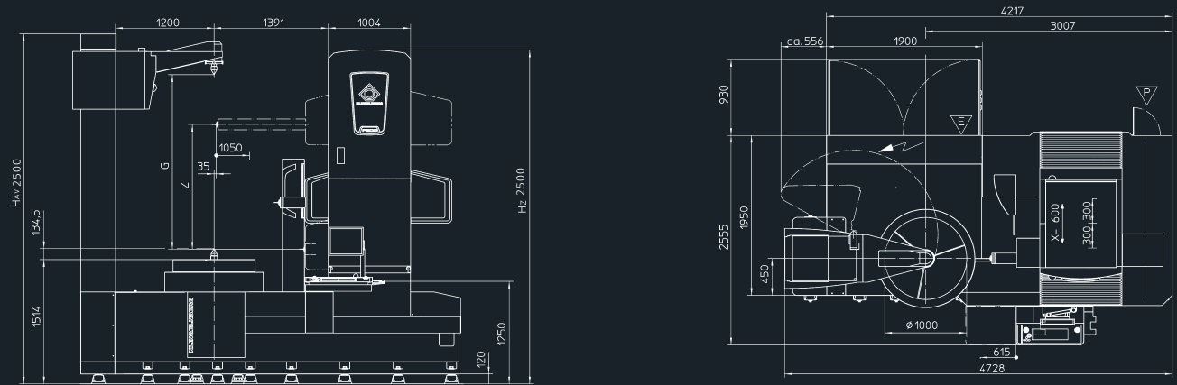
Display with permanently installed column and foldaway counterholder
